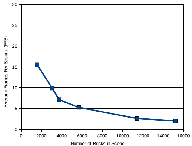
Figure 9: Graphed results of the performance testing of our system. The y-axis shows the number of frames per second, the x-axis the number of trees / bricks in the scene.
